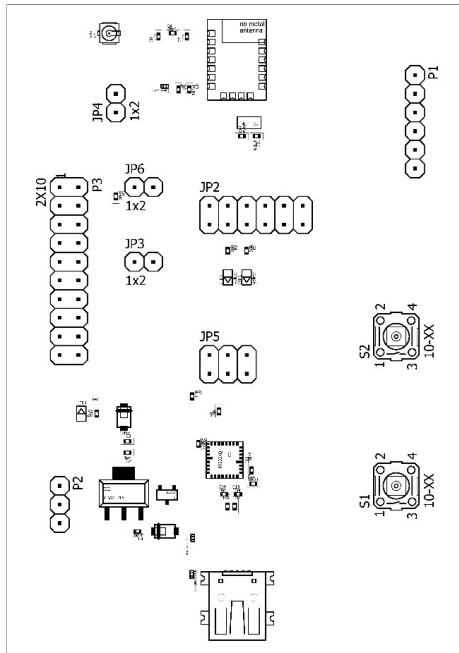
Figure 15: Assembly diagram
