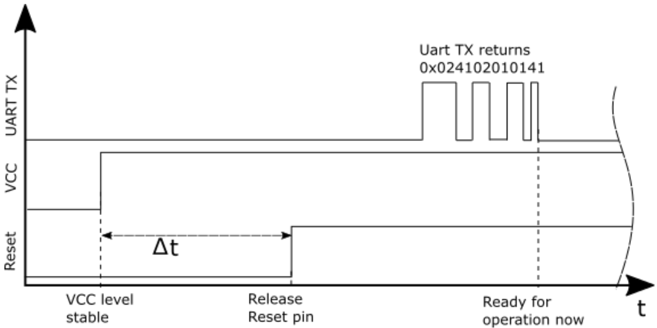
Figure 6: Power up
